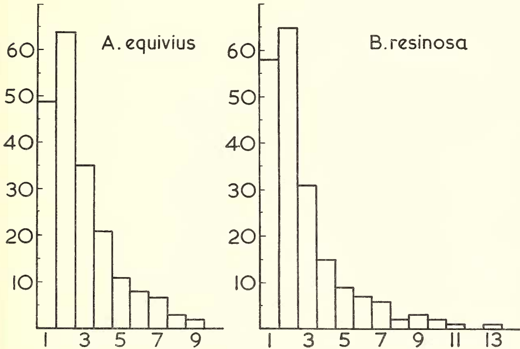
TEXT-FIG. 3. Histograms to show the frequency distribution of the height of 200 rays; A, Amyelon equivius , B, Bilignea resinosa . The height is expressed as the number of cells seen in tangential longitudinal section.
